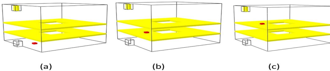
Fig. 6 The effect of changing the location of fire on pressure and temperature is investigated for, (a) fire on the ground floor at a distance of 3.5m, from the wall and aligned with the centers of both side vents, (b) on the same location of point (a), but at the first floor, (c) on the same location of point (a), but at the second floor.
